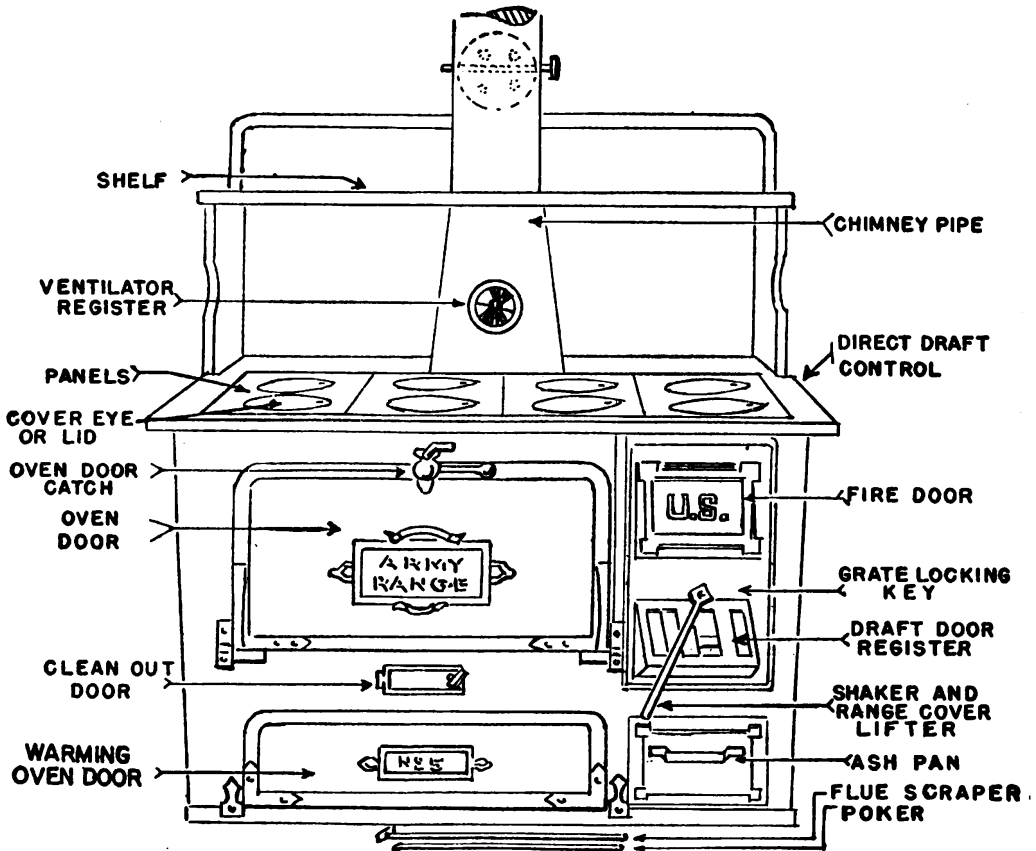
FIGURE 18.1—Army range No. 5.
